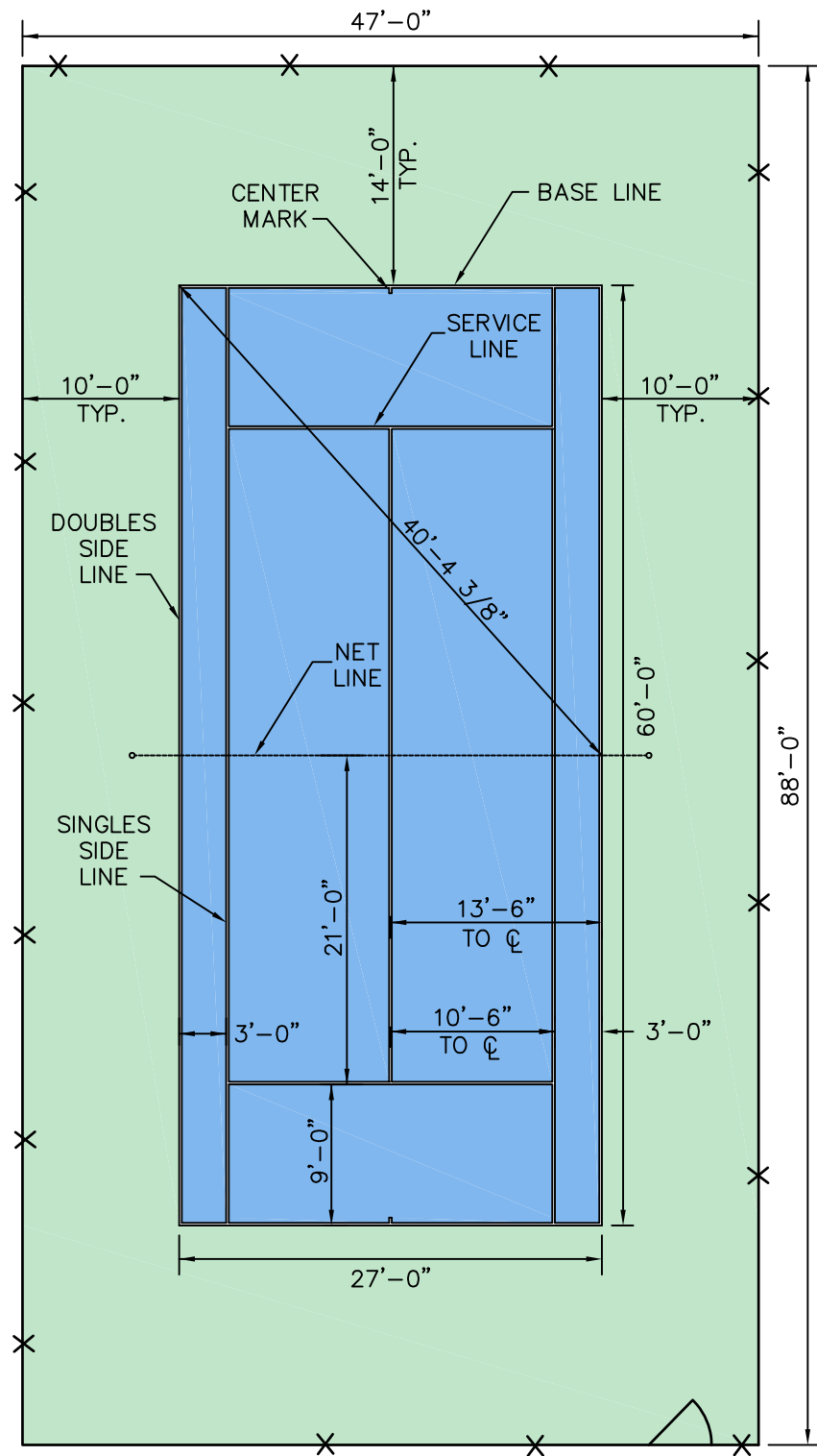
SINGLE COURT LAYOUT (NEW CONSTRUCTION)
