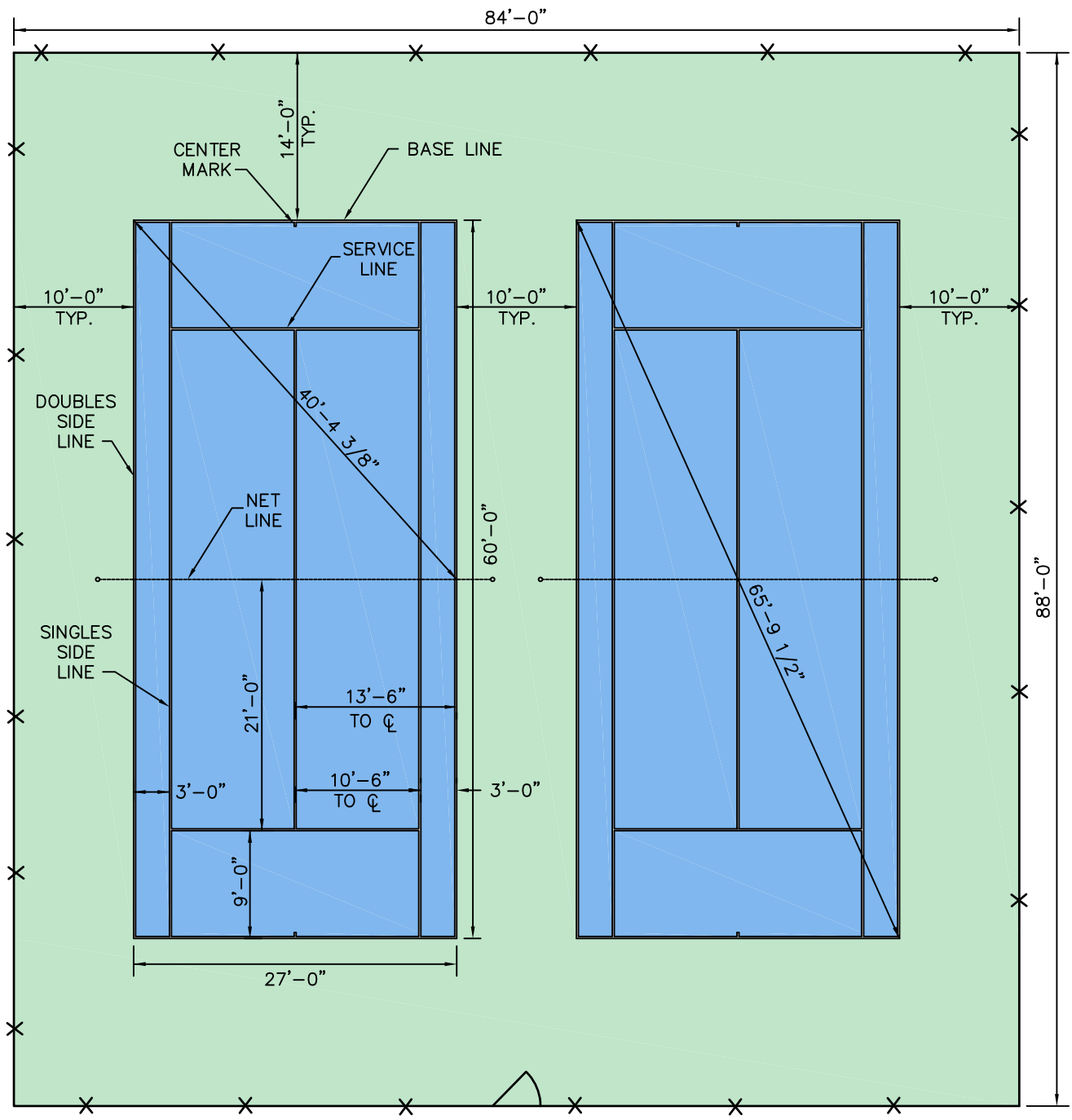
TWO COURT LAYOUT (NEW CONSTRUCTION)
